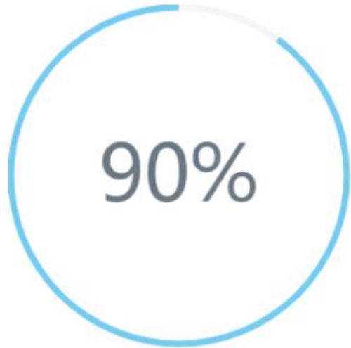
Arrival Rate
