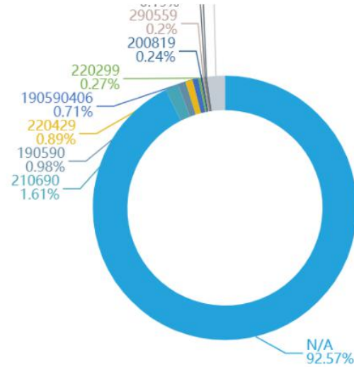
Proportion
